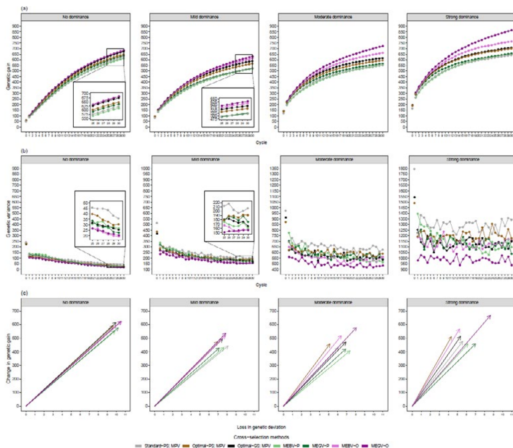
Figure 1: The evolution of genetic gain (a) and genetic variance (b) for a target trait along 30 breeding cycles on average across 30 simulation runs. The efficiency of converting genetic diversity into genetic gain (c) by regressing the change of genetic gain on the loss of genetic standard deviation between cycle 0 and cycle 30. The three parameters were assessed at D clone stage for different selection strategies (Standard-PS, Optimal-PS, and Optimal-GS), different mean-based cross-selection methods (mean phenotypic values of the two parents [MPV], mean estimated breeding values of the two parents [MEBV-P], mean estimated genetic values of the two parents [MEGV-P], mean estimated breeding values among simulated offspring [MEBV-O], and mean estimated genetic values among simulated offspring [MEGV-O]), and different genetic architectures of the target trait (no, mild, moderate, and strong dominance effects).
