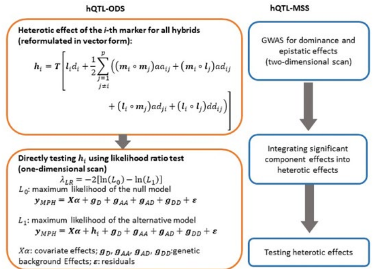
Figure 2: Overview of the principle of the one-dimensional scan (hQTL-ODS) developed for heterotic QTL, compared to the existing multi-step approach (hQTL-MSS).
