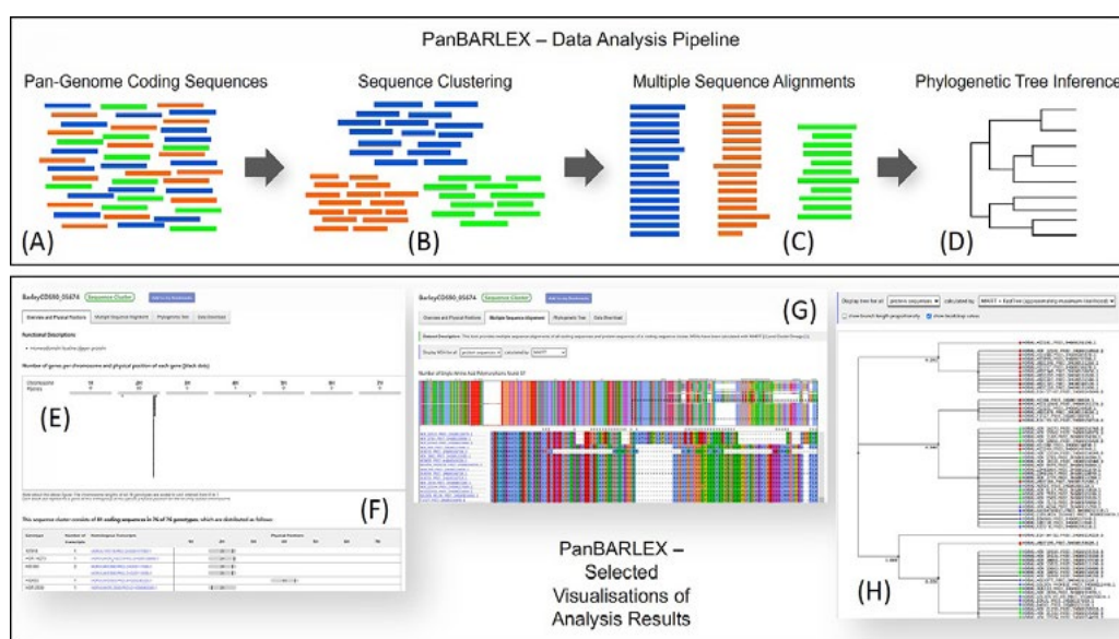
Figure 1: Overview about the PanBARLEX data analysis pipeline (A – D) and selected visualisations of the analysis results (E – H). As input the pan-genome coding sequences of 3,797,824 annotated genes were used (A). Using MMseqs2 a sequence clustering was carried out (B). The results were used as input to precompute multiple sequence alignments using MAFFT and Clustal Omega (C). These results are used as input to compute phylogenetic tree inferences using FastTree and Clustal Omega (D). Sequence cluster visualisation using the example of the cluster of the gene “Vrs1” are visualised in part (E – F) where (E) recognises the spatial distribution of homologous genes across all chromosomes and (F) shows the presence-absence variation and copy number variation of homologous genes for all 76 genotypes. (G) illustrated the online viewer for the precalculated multiple sequence alignments for selected sequences clusters generated in step (C). The results of step (D) are visualised in an interactive phylogenetic tree viewer (H).
