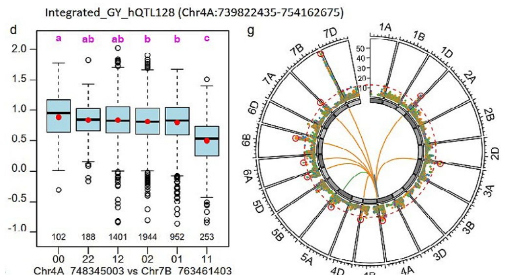
Figure 3: Heterotic QTL detected for grain yield on chromosome 4A (Integrated_GY_hQTL128). The phenotypic distribution of grain yield MPH for hybrids with distinct genotype combinations of the peak SNP within hQTL and the SNP showing the most significant epistatic interaction effect with the peak SNP. Circled Manhattan plot of epistatic effects between the peak SNP of hQTL and all other SNPs.
